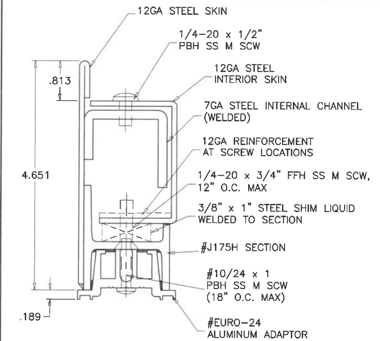
8 PANEL STD. BOTTOM RAIL ASSEMBLY
