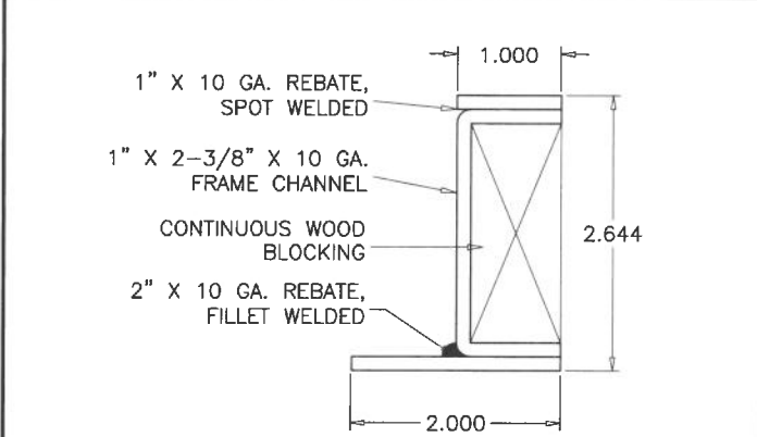
3 LOCK JAMB ASSEMBLY
