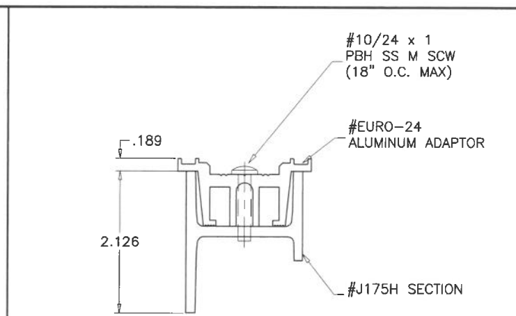
6 PANEL PIVOT STILE ASSEMBLY
