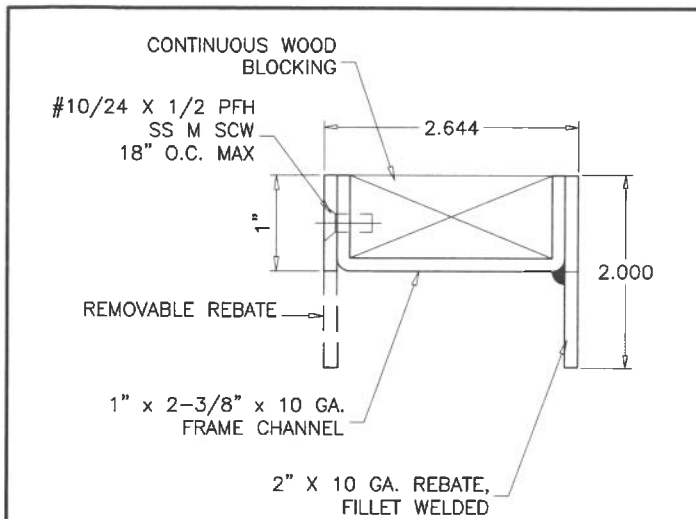
1 FRAME HEAD ASSEMBLY
