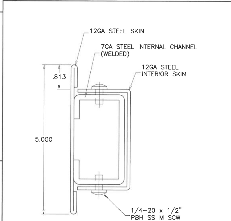
5 PANEL TOP RAIL ASSEMBLY
