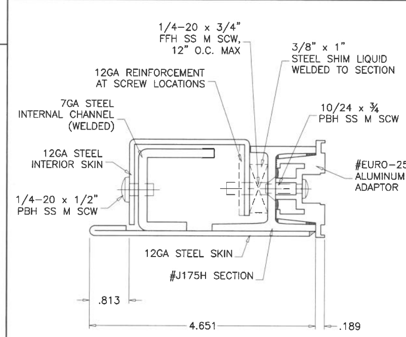
6 PANEL PIVOT STILE ASSEMBLY
