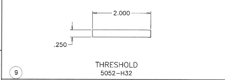
24 MID-RAIL ASSEMBLY
