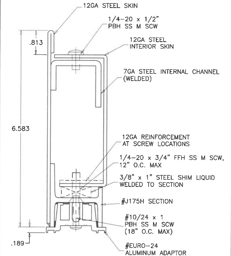
8A PANEL HIGH BOTTOM RAIL ASSEMBLY
