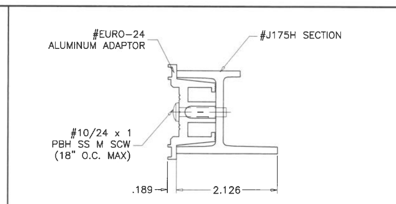
6 PANEL PIVOT STILE ASSEMBLY
